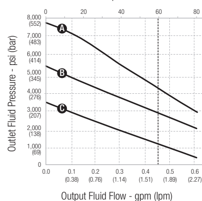
Dyna-Star 70:1 Pump Performance Curve Air Motor Speed — CPM
