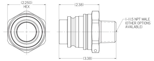
FF5-SERIES NIPPLE
