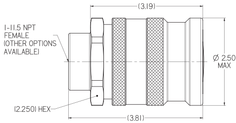
FF0-SERIES SOCKET
